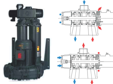
VS SERIES FLOW REVERSING VALVE
