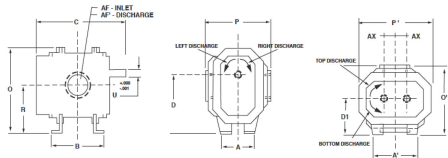
RAM SERIES rotary positive blowers frames 404 thru 624
