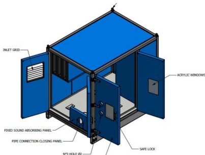
Small Bag dumping station
