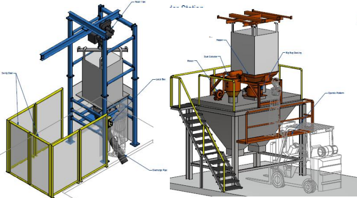
Big Bag & Tote bin Unloading Station
