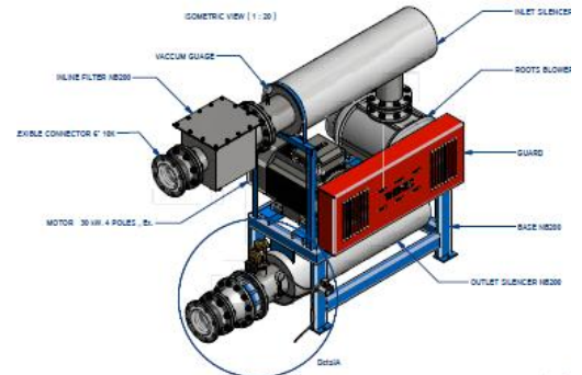
Acoustic Enclosure & Blower package
