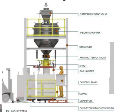
Big Bag Filling & Weighting Station
