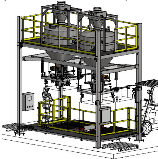
Big Bag Filling & Weighting Station / High & Low Speed / Platform Scale & Hopper scale
