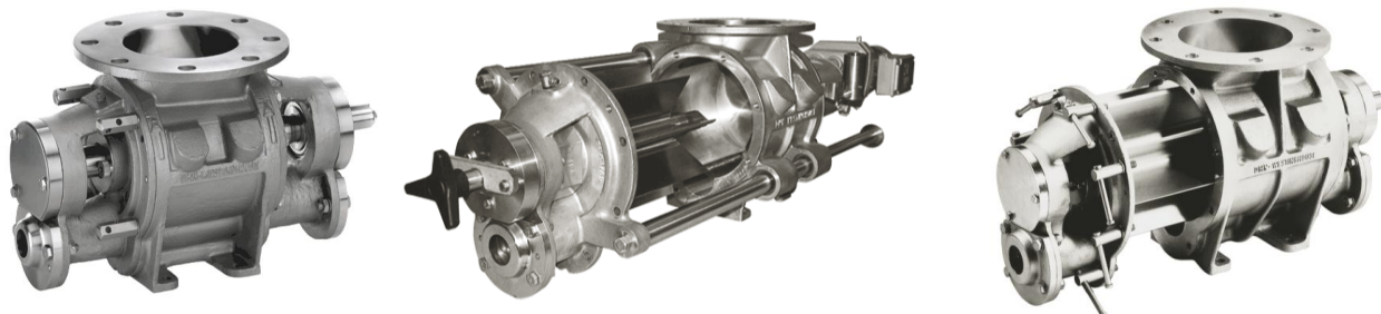
Blow Through Rotary valve / normal , quick detachable and dairy valve type
