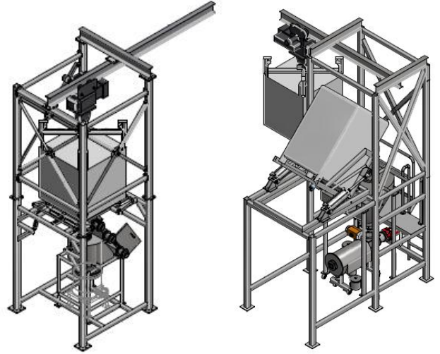
Big Bag & Tote bin Unloading Station
